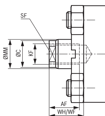
Internal thread "E"
