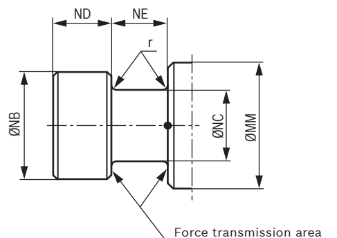
Trunnion "T"
